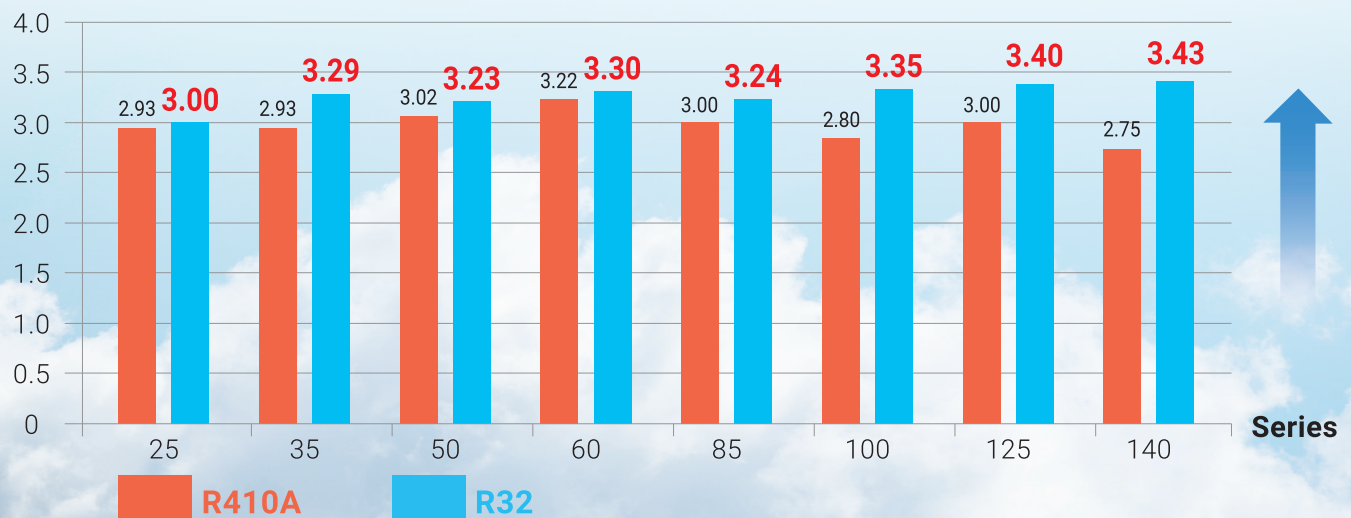
COP(W/W)
