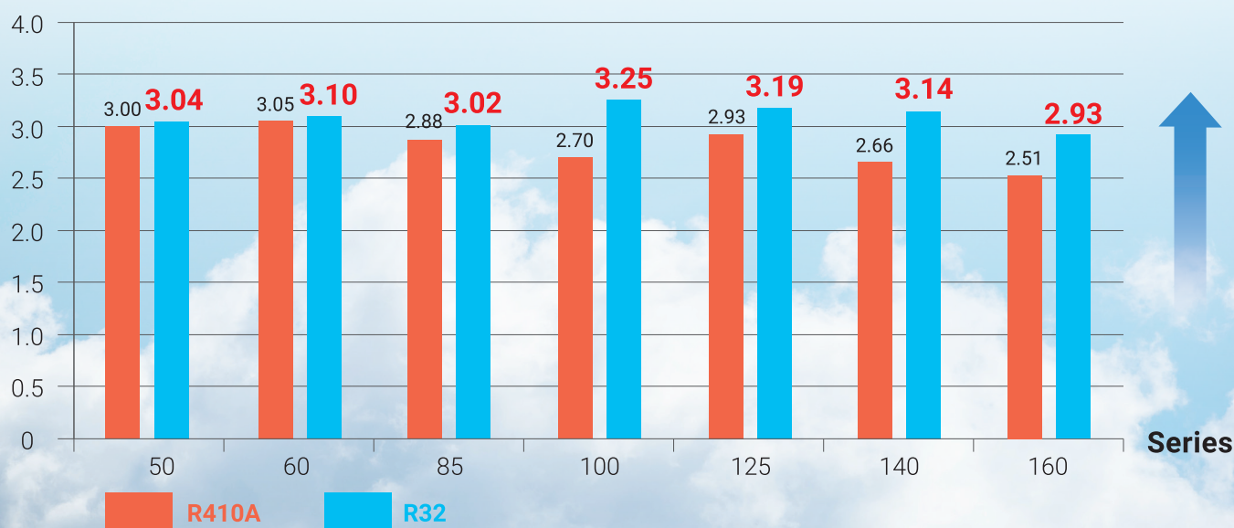
COP(W/W)
